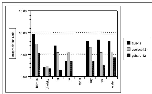
Figure 18: 2 threads, BTB of 1024 entries, PHT of 8k entries
