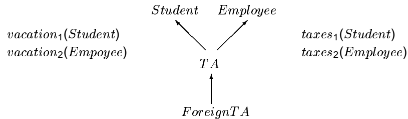
Figure 3: Example Type Hierarchy and Methods
