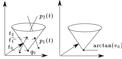
Figure 3: The postmen in (x, y, t) space and the cone C_q of the dog's motion options
