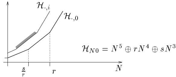
Figure 1: A series with large weak rank
