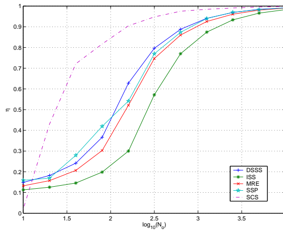
Fig. 9. WOA for five different watermarking methods ( N_v = 512 , N_c = 4 , WCR = -15\text{dB} ). \tau = 128 for SCS. For SCS, SSP and ISS, the embedding parameters are optimal for an expected noise attack whose distortion equals the embedding distortion: WNR = 0\text{ dB} .
