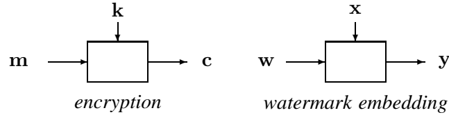
Fig. 3. An analogy with cryptography: plaintext \mathbf{m} \rightarrow watermark \mathbf{w} , key \mathbf{k} \rightarrow original \mathbf{x} , ciphertext \mathbf{c} \rightarrow watermarked content \mathbf{y} .
