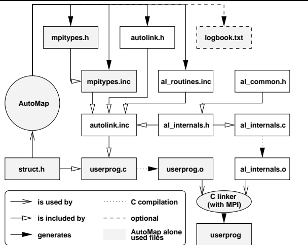
Figure 3 AutoMap and AutoLink files generation; struct.h is the user type definition file, userprog.c is the C source that uses the output of AutoMap/AutoLink
