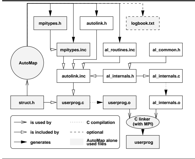
Figure 3 AutoMap and AutoLink files generation; struct.h is the user type definition file, useprog.c is the C source that uses the output of AutoMap/AutoLink
