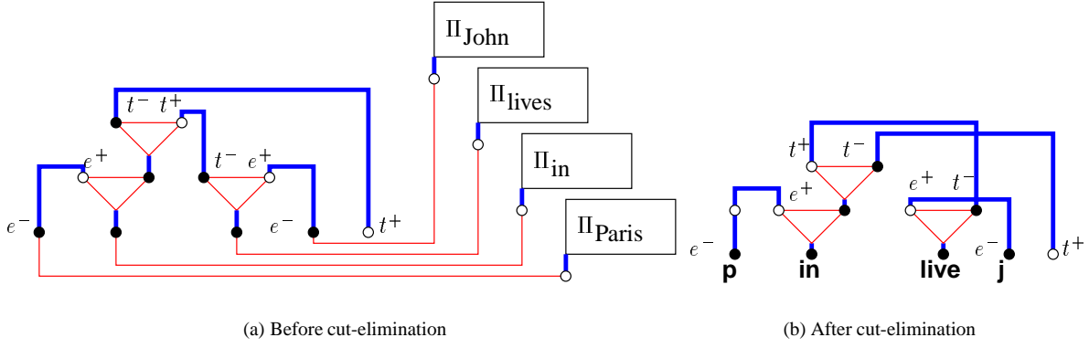
Figure 4: Semantic proof nets for (in p)(live j)
