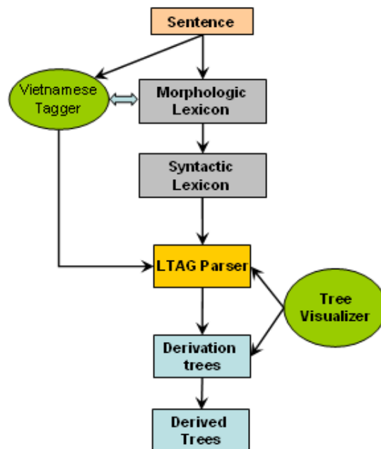
Figure 7: The parsing scheme for Vietnamese
