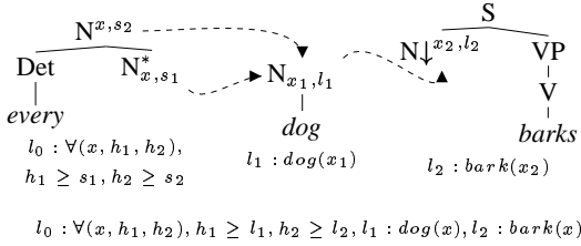
FIG. 3 – Quantifiers
