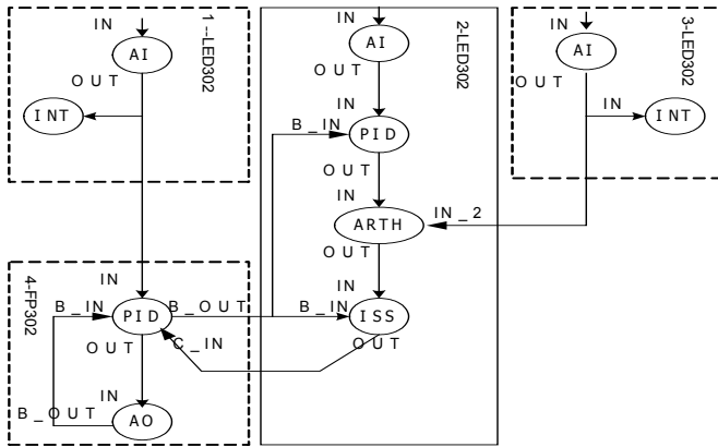
Fig 9 Control Strategy of Boiler Water level Control System
