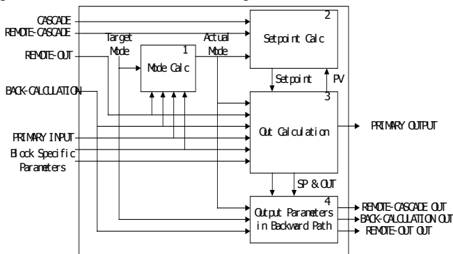
Fig 3 IEC FB Operation Procedure
