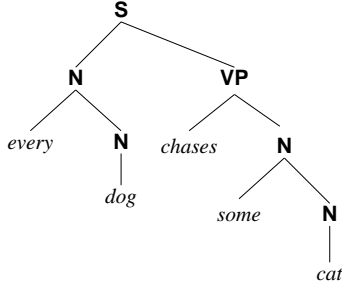
Figure 2: \mathcal{L}(c_{chases} I_S I_{VP}(c_{dog} c_{every})(c_{cat} c_{some})) = \mathbf{S}_2(\mathbf{N}_2 \text{ every } (\mathbf{N}_1 \text{ dog}))(\mathbf{VP}_2 \text{ chases } (\mathbf{N}_2 \text{ some } (\mathbf{N}_1 \text{ cat})))
