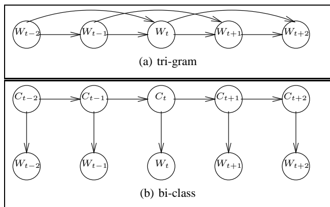
Figure 1: tri-gram and bi-class models
