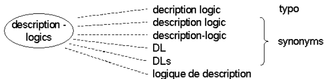
Figure 3. Grouping keywords
