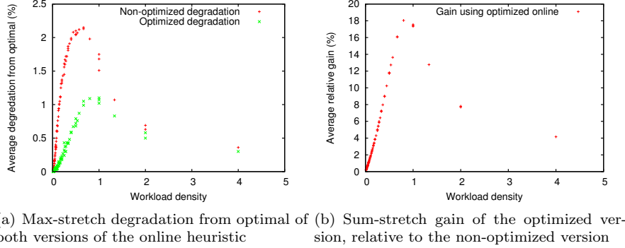
Figure 10: Comparison of the optimized and non-optimized versions of the online heuristic.
