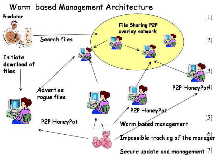
Fig. 6. Worm based management : a case study
