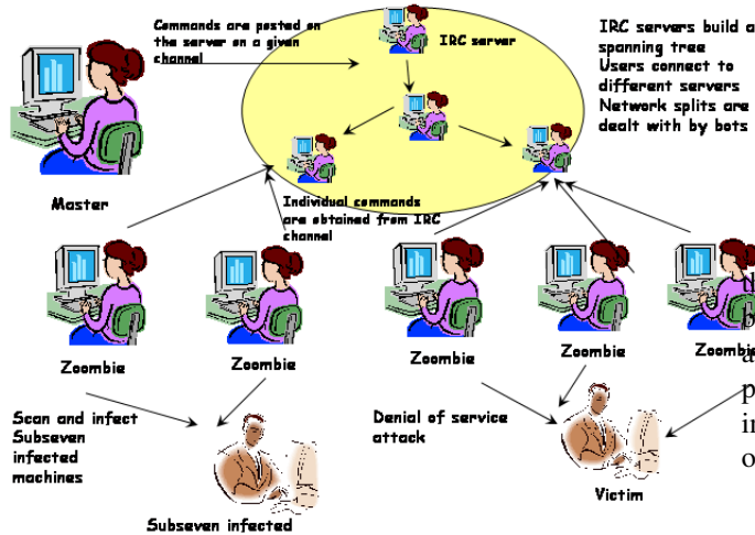
Fig. 3. IRC based worms
