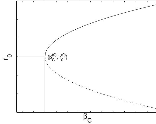
Figure 3: Schematic plot of the positions of the extrema of the energy of a circle versus \beta_C .
