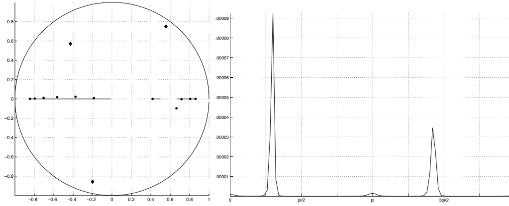
Figure 2. Poles of \Pi_{20} the error |F - \Pi_{20}| on \mathbb{T}
