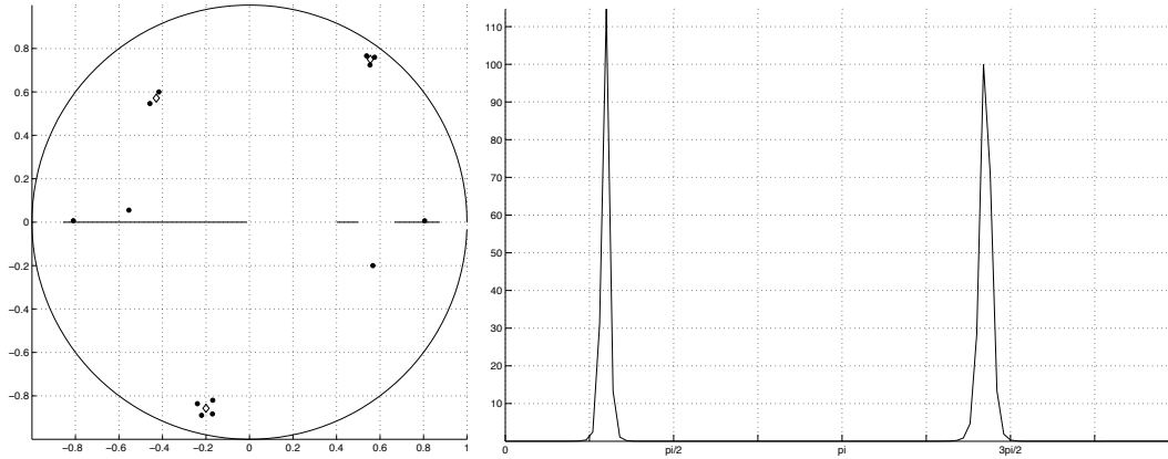
Figure 1. Poles of \Pi_{13} and the error |F - \Pi_{13}| on \mathbb{T}
