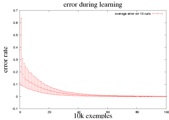
Fig. 4. Error rate during the learning
