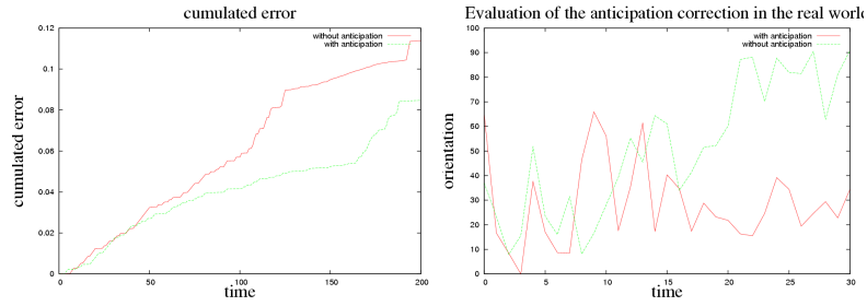
Fig. 10. Real robot error rates. On the left, cumulative error, and on the right, orientation toward the target. The target is centered on approximately 30-40
