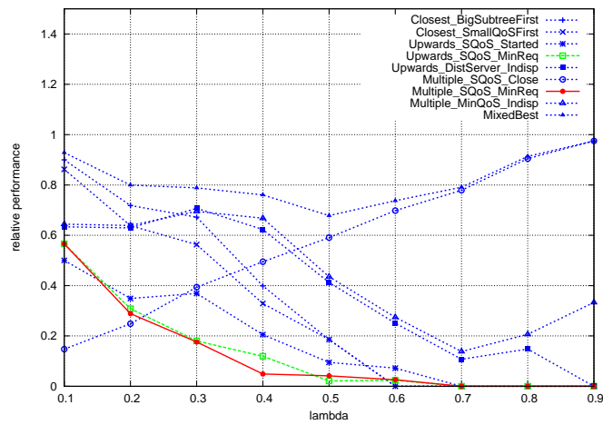
Figure 23: Impact of QoS constraints in small trees, qos = \text{height} + 1 \rightarrow \text{no QoS} .
