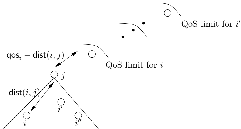
Figure 2: Illustration of the transformation algorithm
