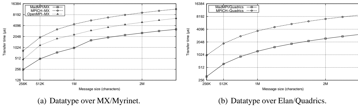
Figure 4: Indexed datatype.
