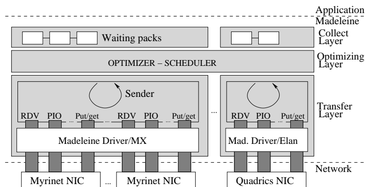
Figure 1: NEWMADLEINE architecture.
