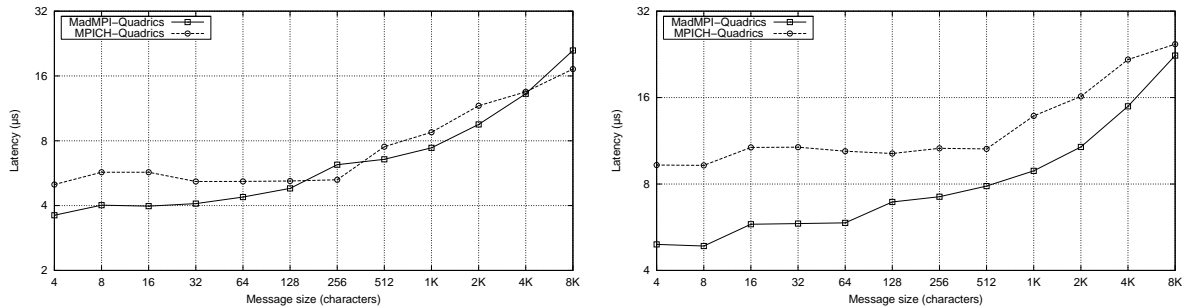
(c) 8-segments ping-pong - Latency over Elan/Quadracs. (d) 16-seg. ping-pong-Latency over Elan/Quadracs.
