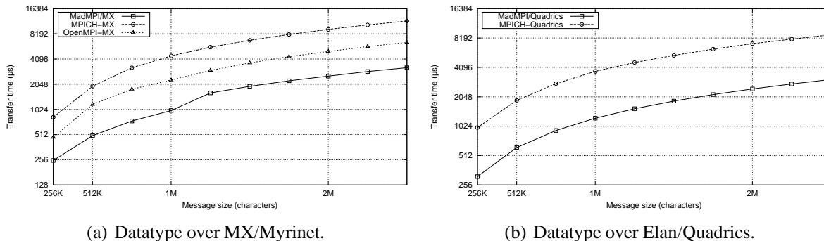
Figure 4: Indexed datatype.
