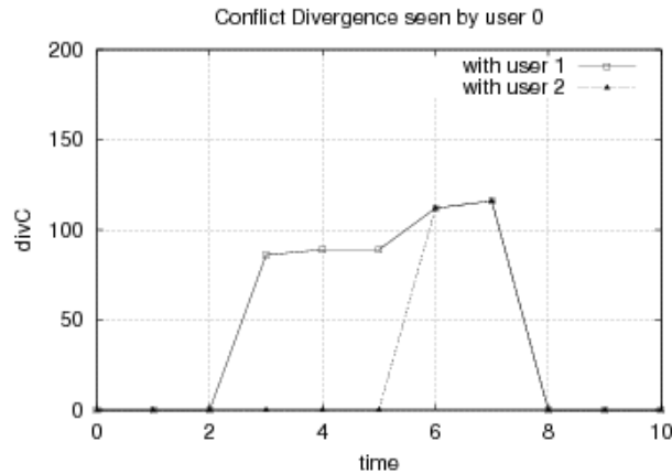
Figure 4. Divergence metric
