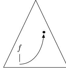
Fig. 4. f(\text{pos}(-n, \dots))
