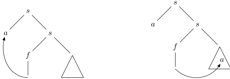
Fig. 7. \text{deref}(a()) ambiguity
