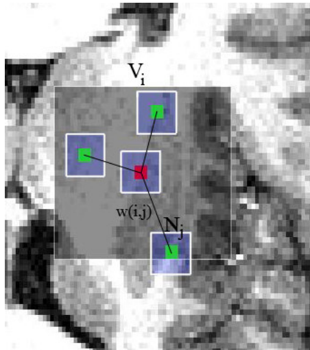
Fig. 1. 2D illustration of the NL-means principle. The restored value of voxel i (in red) is a weighted average of all intensities of voxels j in the search volume V_i , according to the similarity of their intensities neighborhoods v(N_i) and v(N_j) .
