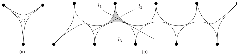
Figure 22: (a) A piecewise-concave polygon P that cannot be guarded solely by vertex guards. Two consecutive edges of P have a common tangent at the common vertex and as a result the three vertices of P see only the points along the dashed segments. (b) A piecewise-concave polygon P that requires 2n - 4 point guards in order to be guarded.
