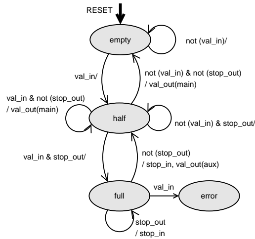
Figure 4: Relay-Station synchchart
