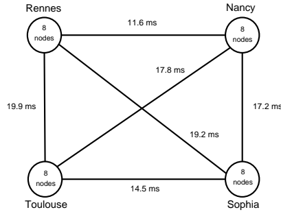
Figure 8: RTT times between each site for the execution of ray2mesh
