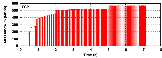
(a) Impact of the slowstart on TCP
