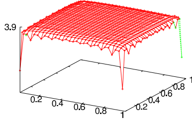
Fig. 2.1: min-cut with IRON only, on a lattice
