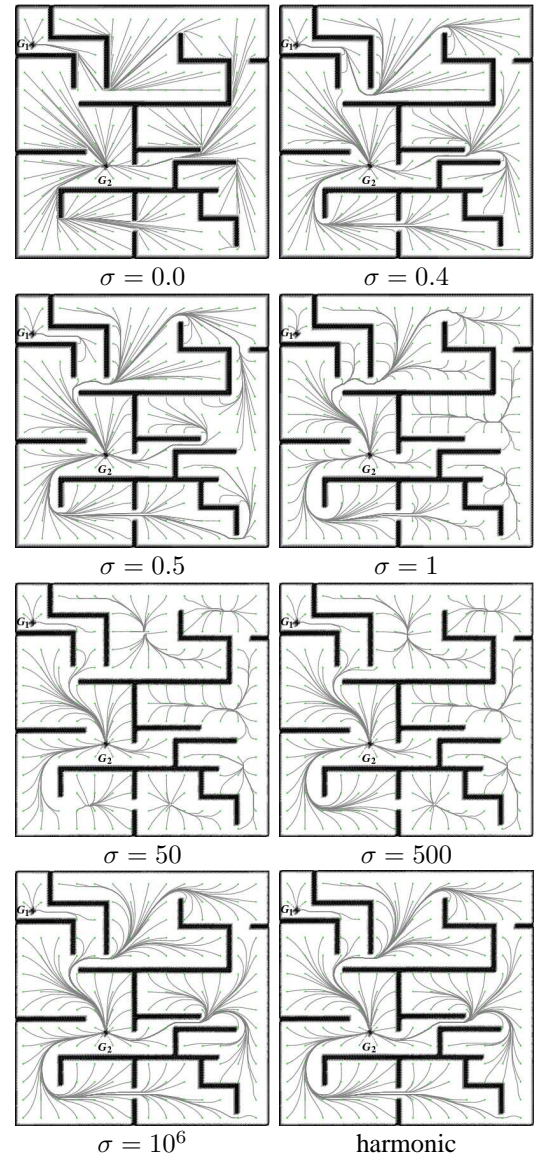
Fig. 2. Evolution of trajectories with respect to the noise level \sigma . Each figure illustrates different trajectories leading to goals G_1 and G_2 , and starting at equally distributed grid points in the environment. All trajectories were computed using optimal control (with J_\sigma^\delta ) except the last one which is derived from harmonic control (with \Phi^\delta ).
