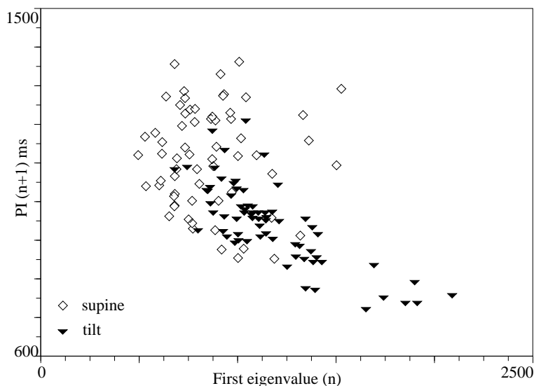
Figure 8: Beat-to-beat BRS, represented as the relation between |\lambda_1(n)| and PI(n + 1) . Slope and correlation are stronger during tilt.
