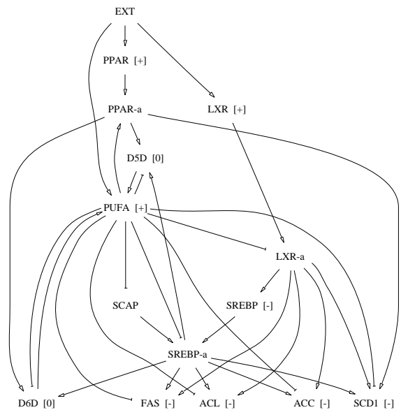
Figure 4. Interaction graph for a model of regulation of the synthesis of fatty acids. The node EXT represents the exterior world. Negative self-interaction loops on nodes are omitted for sake of clarity. Labelled loops: l_1^- = \{PUFA, SCAP, SREBP, D6D, PUFA\} , l_2^- = \{PUFA, SREBP, D6D, PUFA\} , l_3^- = \{PUFA, LXR, SREBP, SREBP, D6D, PUFA\} , l_4^- = \{PUFA, D6D, PUFA\} , l^+ = \{PUFA, PPAR, D6D, PUFA\} . Labelled paths p = \{PUFA, LXR, SREBP\} , p' = \{LXR, LXR, SREBP\} , p_1 = \{PUFA, D6D\} , p_2 = \{PUFA, SCAP, SREBP, D6D\} , p_3 = \{D6D, PUFA\} , p_4 = \{PUFA, LXR, SREBP, SREBP, D6D\} , p_5 = \{LXR, LXR, SREBP, SREBP, D6D\} , p_6 = \{PPAR, PPAR, D6D\} , p_7 = \{PUFA, PPAR, D6D\} , p_8 = \{PUFA, SREBP, D6D\} , p_9 = \{PPAR, PPAR, D6D, PUFA\} , p_{10} = \{LXR, LXR, SREBP, SREBP, D6D, PUFA\} .
