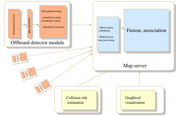
Fig. 2. The ParkView platform software organization
