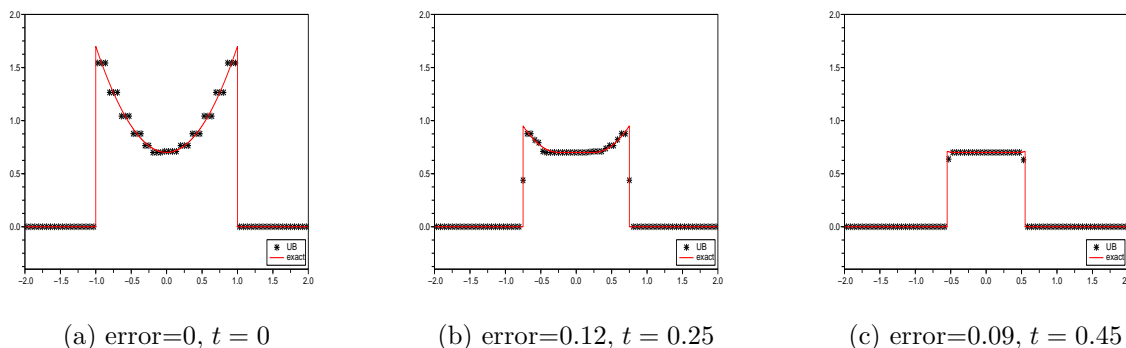
Figure 7: (Example 3) Piece wise continuous function with two maxima, # cells=70.
