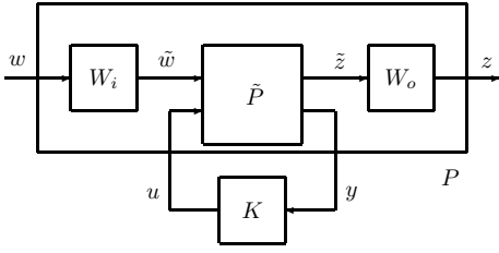
Fig. 3. Focused interconnection
