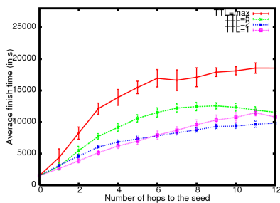
Fig. 3. Average finish time as a function of number of hops to seed for different flooding scope
