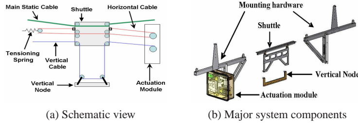
Fig. 2: NIMS system with basic cable setup
