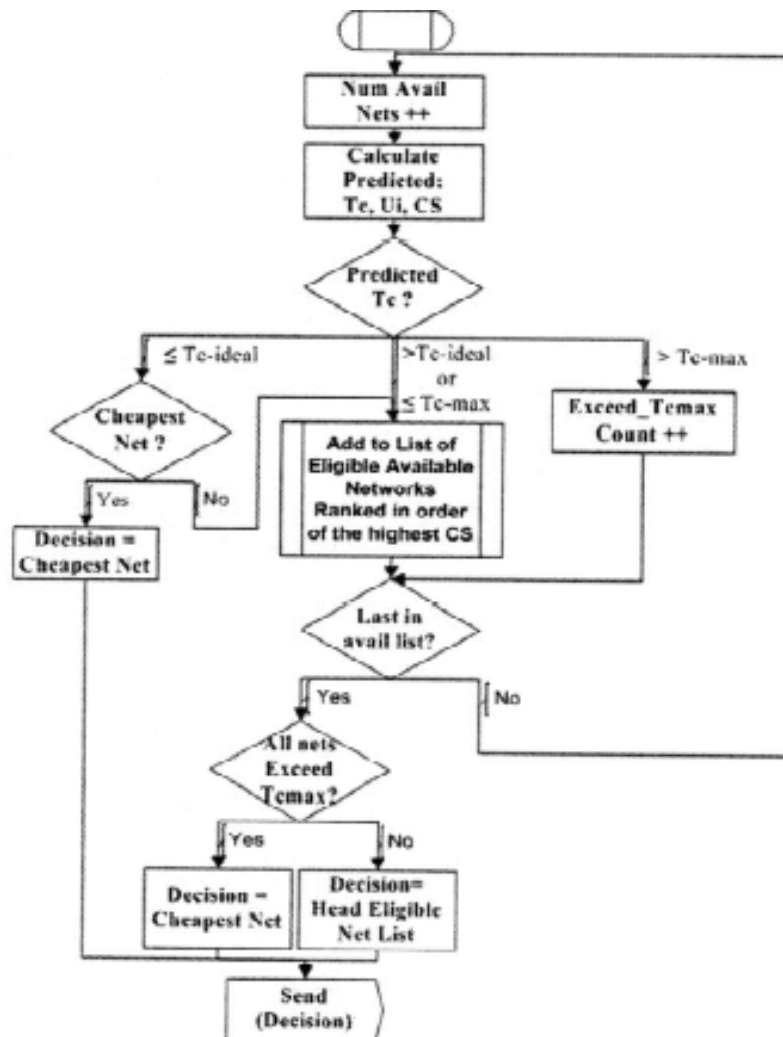
Figure 7: Decision strategy based on predicted T_c
