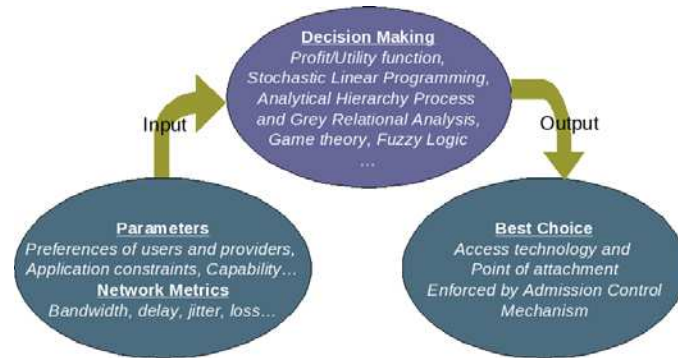
Figure 3: Decision making: input, processing, and output
