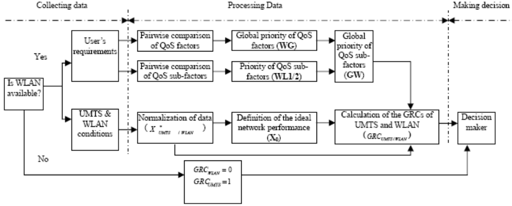
Figure 12: AHP and GRA based network selection model
