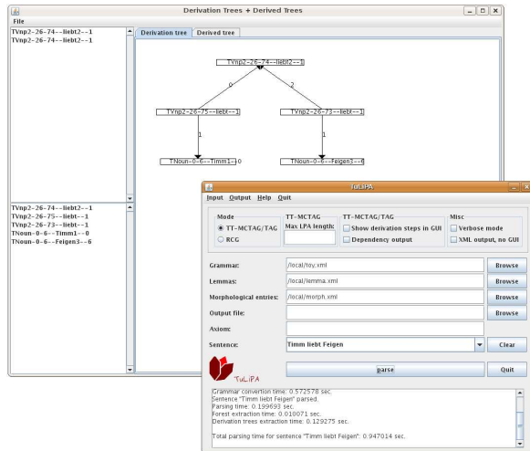
Figure 5: TuLiPA's Graphical User Interface.
