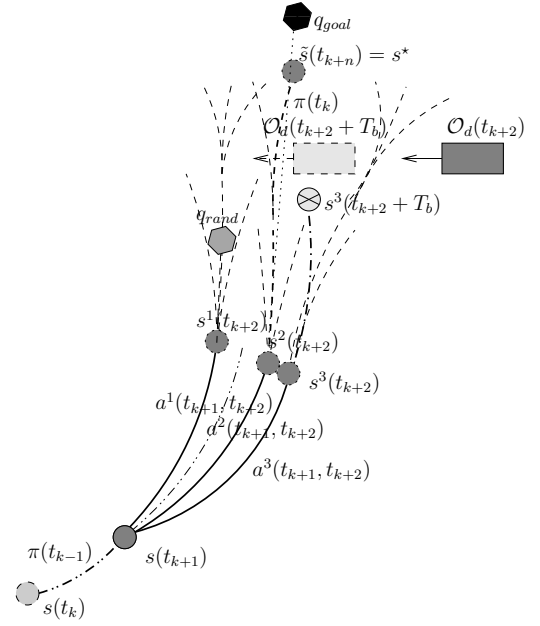
Fig. 4. Node expansion
