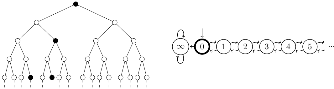
Figure 4: The Dyck tree and its minimal graph.
