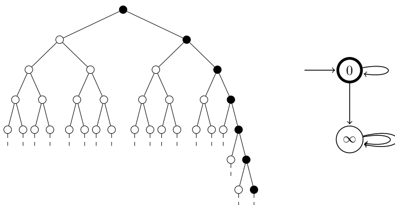
Figure 2: A tree T and the associated minimal multi-graph G(T) .
