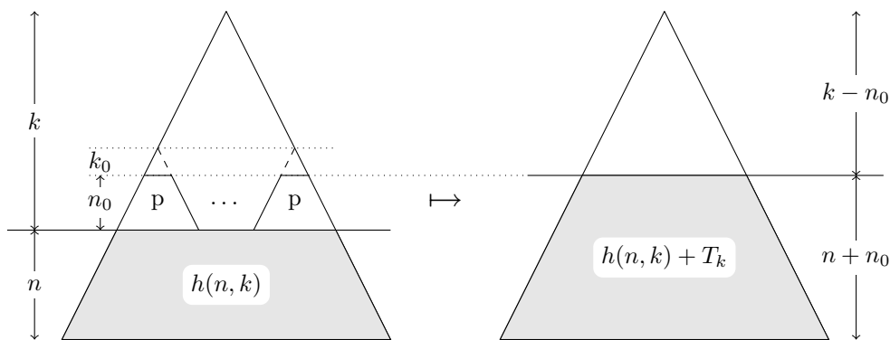
Figure 11: The first transformation: if k > n_0 + k_0 , we add a level of factors of shape n_0, k_0 that all contain exactly p ones. The shape of the factor becomes (n + n_0, k - n_0) . We repeat the transformation until the shape is (n', k') with k' < n_0 + k_0 . In the figure, T_k stands for pd^{k-n_0-k_0}p .
