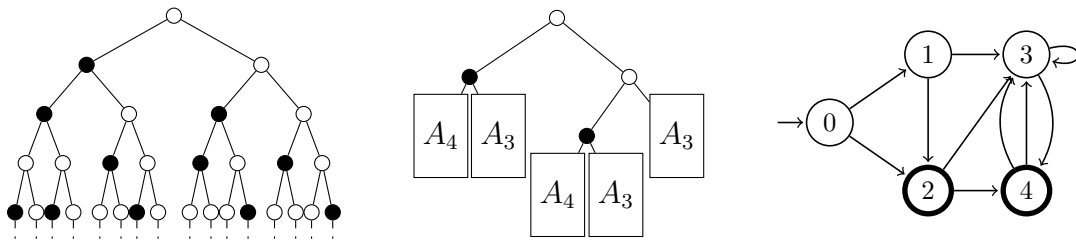
Figure 8: Example of a rational tree that is strongly balanced but not mechanical. On the left is the tree itself. In the middle the mechanical suffixes of the tree are displayed and its minimal graph (reducible) is displayed on the right.
