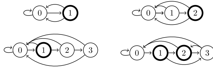
Figure 9: All mechanical trees of the same density \alpha have the same minimal graph G_\alpha . These graphs represent G_\alpha for \alpha = 1/3, 1/7, 4/15 and 6/15 = 2/5 . For all graphs with n nodes, there are exactly n different mechanical trees of this particular density, depending on which node is associated to the root. Note that the first three graphs have a very similar structure (Figure 16 displays more mechanical trees with this structure).
