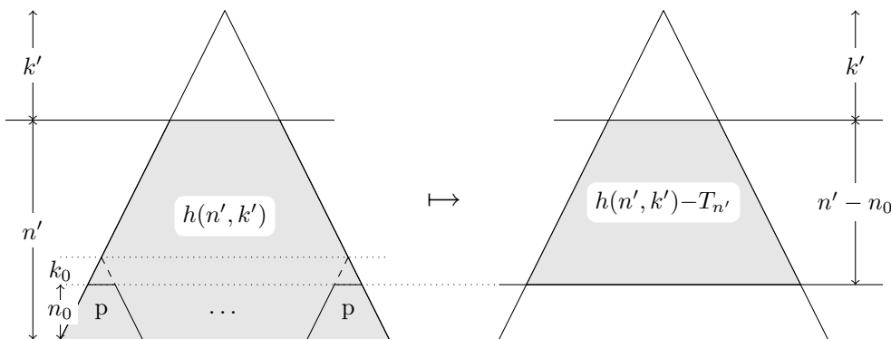
Figure 12: The second transformation: if n' > n_0 + k_0 , we can remove a level of factors of shape (n_0, k_0) . The shape of the factor becomes (n' - n_0, k') . We repeat the transformation until the shape is (n', k') with n' < n_0 + k_0 (here, T_{n'} = pd^{n'-n_0-k_0} ).
