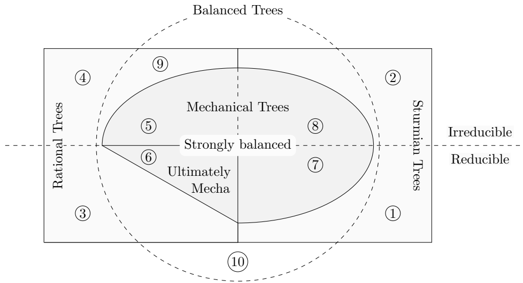
Figure 14: Relations of inclusion linking the different classes of trees. Each number refers to an example detailed in section 6. For example 6 is the set of trees that are rational, reducible, ultimately mechanical, strongly balanced, balanced and neither mechanical nor Sturmian.
