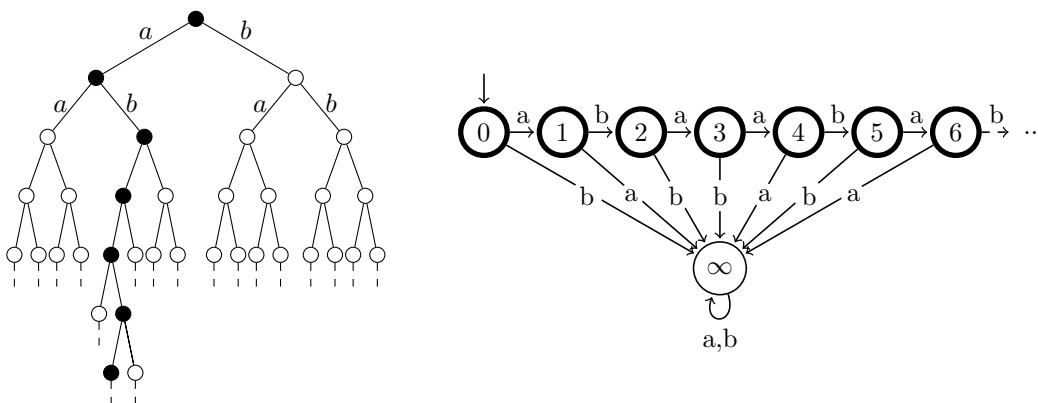
Figure 1: The tree-automaton recognizing the Fibonacci word f and the corresponding minimal automaton. The states of this later are 0, 1, \dots, \infty . There is a transition between nodes i and i + 1 labeled by the i th letter of f and one between nodes i and \infty labeled by the opposite of this i th letter.
