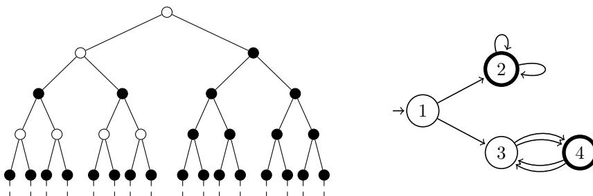
Figure 6: A rational tree made of two distinct subtrees and its associated multi-graph
