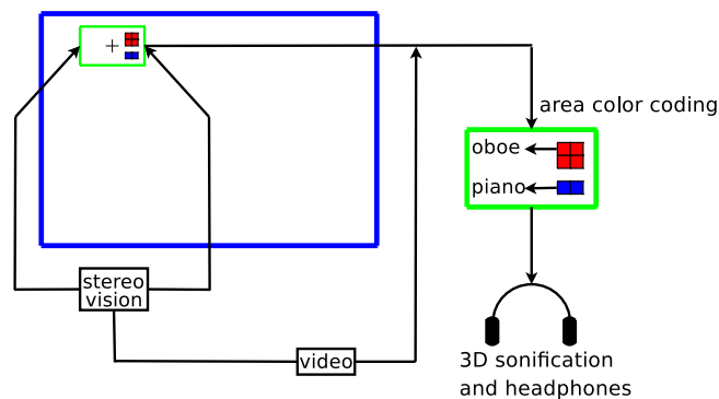
Fig. 1. The See CoLoR general framework.
