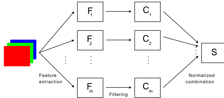
Fig. 3. General overview of the conspicuity map approach for saliency detection. S is the final saliency map, and F_i , C_i the feature maps and their associated conspicuity maps, respectively.
