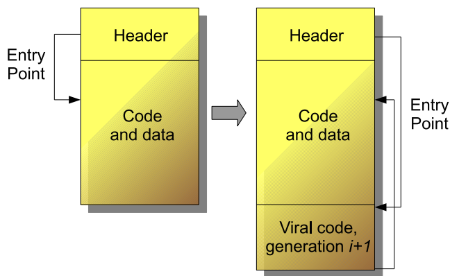
Fig. 3. Metamorphic virus infection on generation i .
