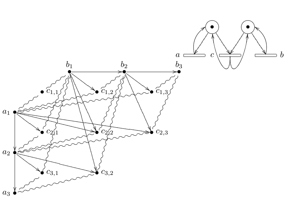
Figure 4: A net with height 0 and infinite branching cells.
