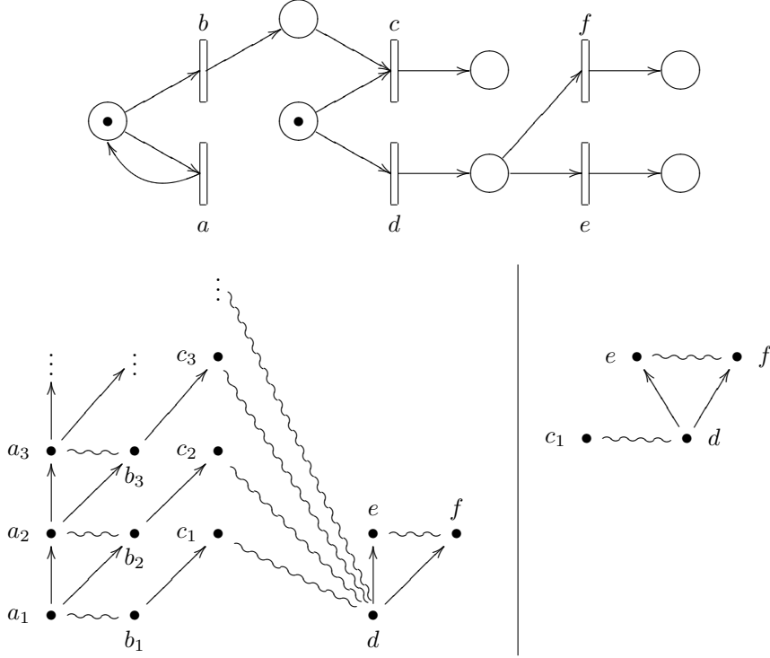
Figure 3: A 1-safe net that unfolds to a non locally finite event structure.
