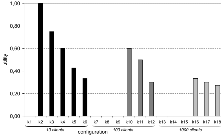
Figure 3: Utility function
