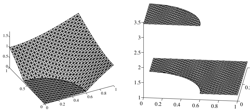
Fig. 4. Elevation of |u| and p for \nu_1 = 0.49 .
