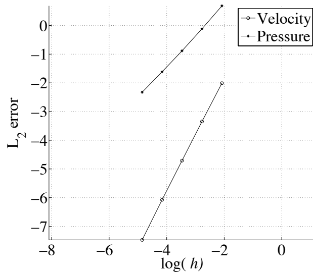
Fig. 1. Convergence for an artificial interface.
