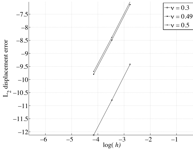
Fig. 3. Convergence for the elasticity problem.
