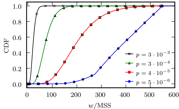
FIG. 14 – Distribution of Y_n for TCP Reno ( \mu\bar{\tau} = 400 MSS)
