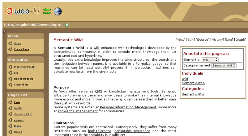
Figure 6: P-Swooki Interface
