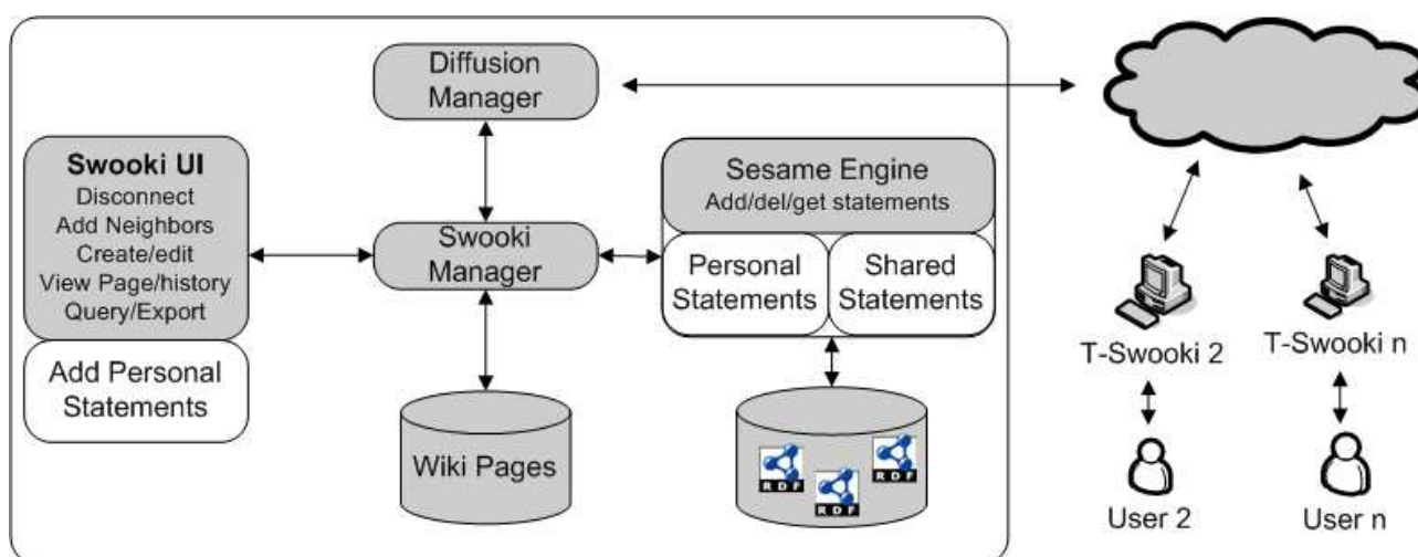
Figure 5: P-Swooki Architecture
