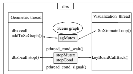
Figure 1: Geometric and visualization threads under the debugger
