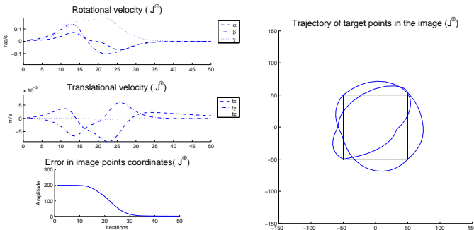
Fig. 2. Convergence using J^\oplus for a 180° rotation around the optical axis
